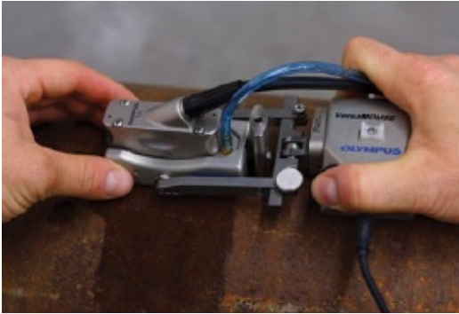
VersaMOUSE scanner and RexoFORM for corrosion inspection.
