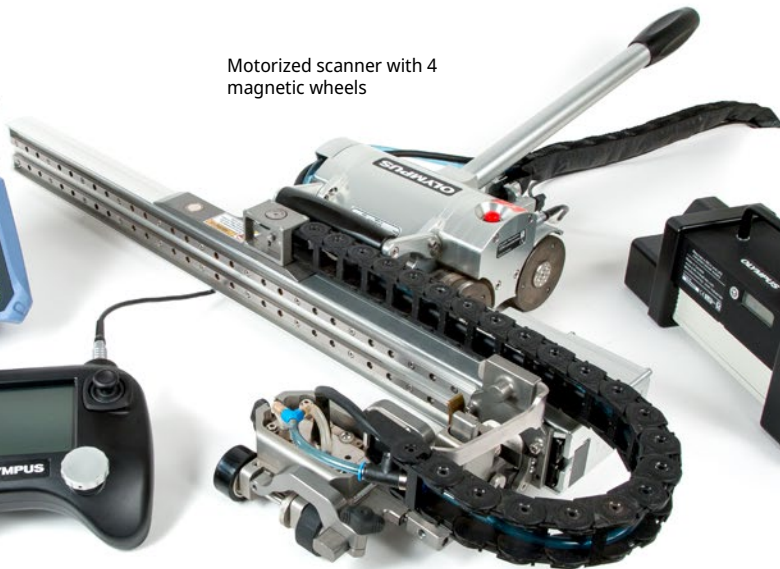
HydroFORM scanner and holder assembly
