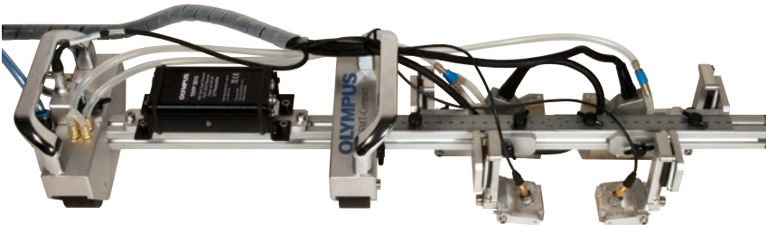
This configuration is suitable for hard-to-reach places, such as pipe-to-component welds.
